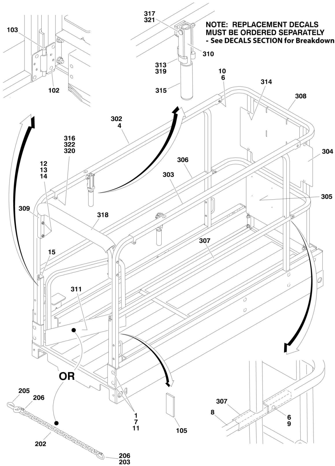
FIGURE 4-2. RAIL (FIXED) INSTALLATION - 1930ES
